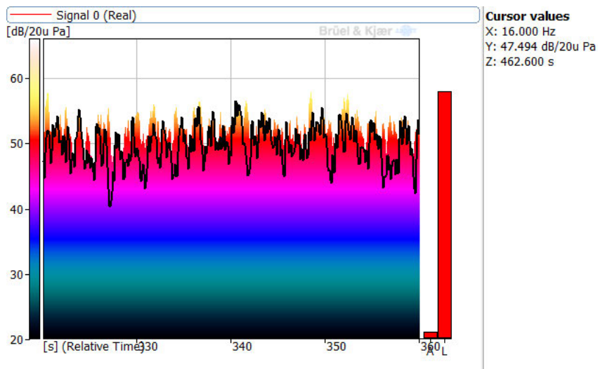
Figure 5: 16 Hz 1/3 octave band time signal relative to reported sleep disturbance for Figure 4
