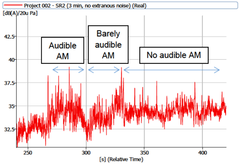
Figure 6: A-weighted time trace – Capital Windfarm
