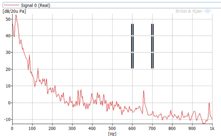
Figure 4: FFT relative to reported sleep disturbance (24 Oct 2016)
